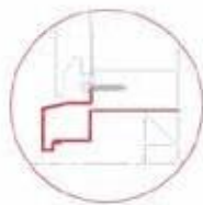
6. Remat superior finestra
